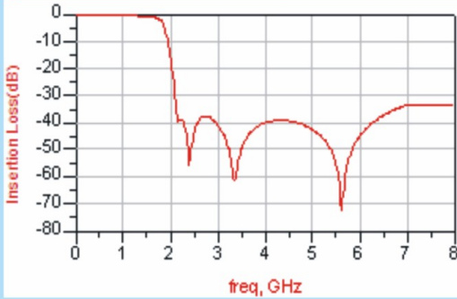
● LFCN3216-1500A01
