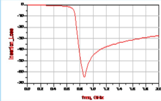
● LFCN3216-520A01*
