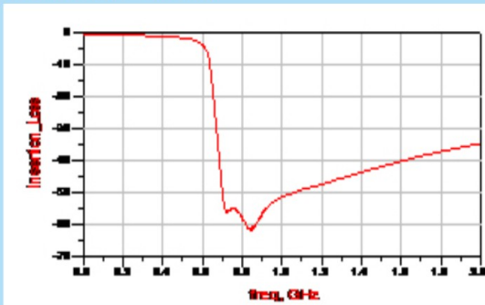
● LFCN3216-420A01
