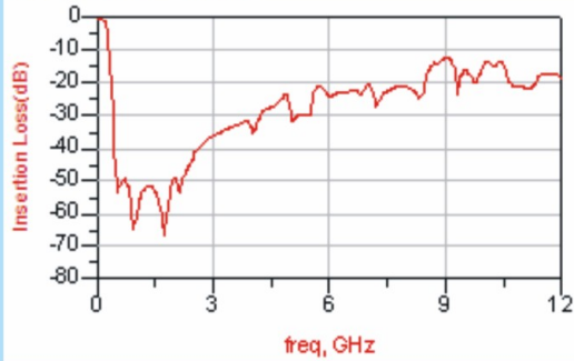
● LFCN3216-180A01
