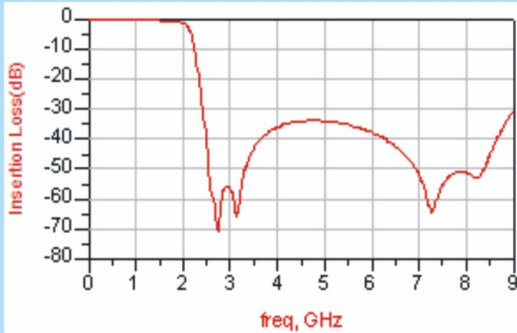
● LFCN3216-1800A01
