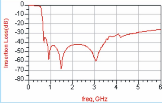
● LFCN3216-400A01
