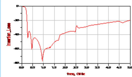
● LFCN3216-100A01
