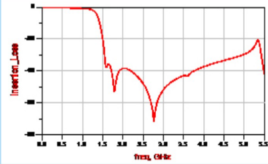
● LFCN3216-1000A01
