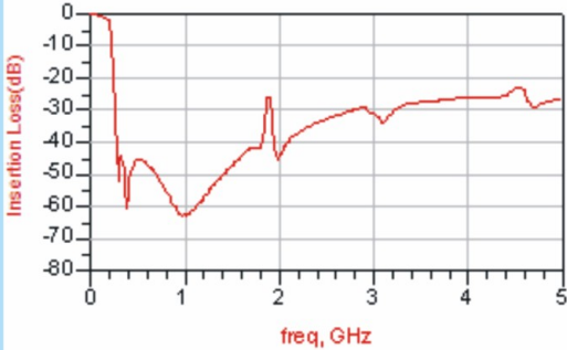
● LFCN3216-120A01
