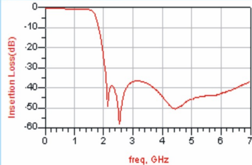
● LFCN3216-1450A01
